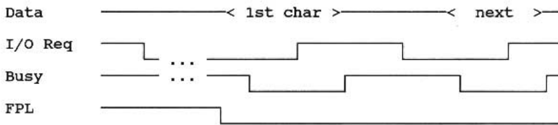
Figure 16.4 Message Output During Immediate Handshake (CY545B drives data)
