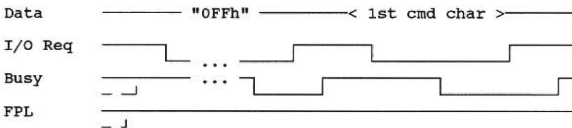
Figure 16.5 Normal Immediate Handshake or Continued Handshake after msg
