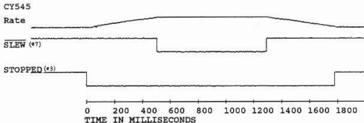
Figure 16.13 SLEW signal waveform.
