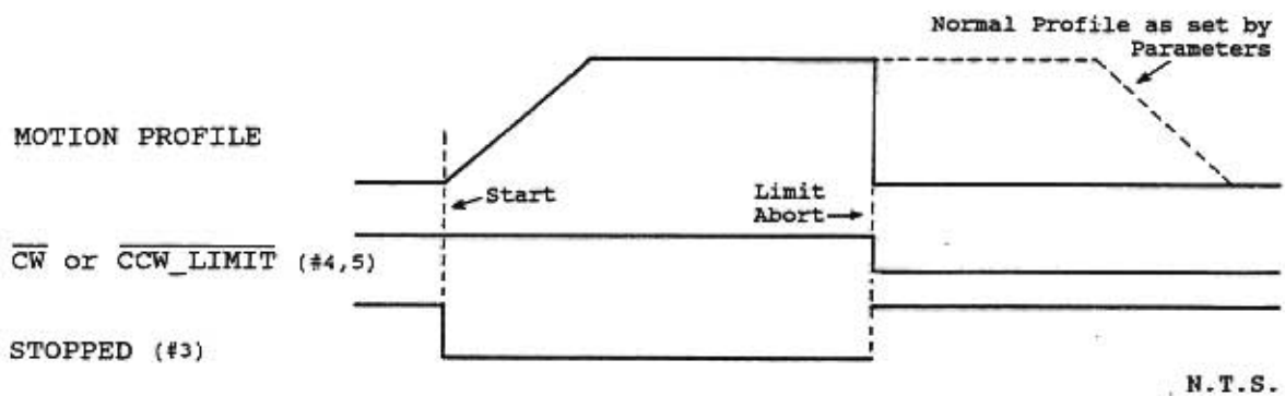
Figure 16.16 CW_LIMIT or CCW_LIMIT signals stop a motion.
