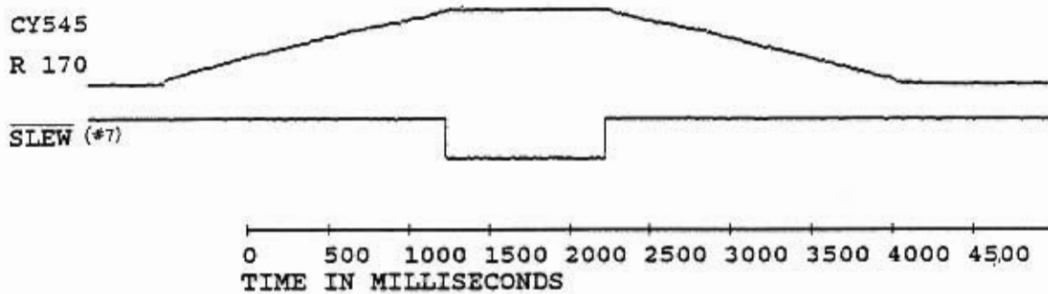
Figure 17.1 Optimal acceleration curve
