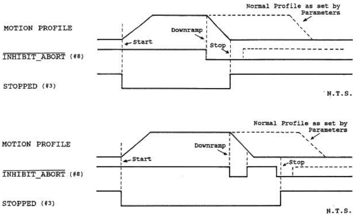
Figure 16.15 Stopping motions with INHIBIT_ABORT.
