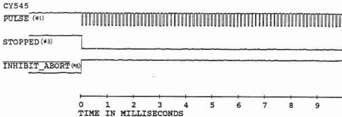
Figure 16.14 INHIBIT_ABORT at the start of motion.
