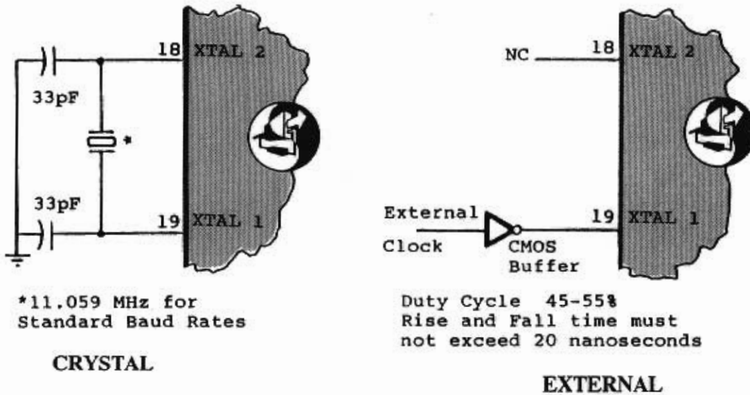
Figure 18.2 Clock Circuits for CY545.
