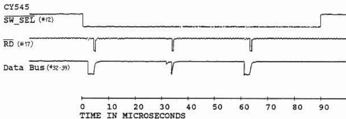
Figure 16.10 Typical Thumb Wheel Switch Parameter Read Waveform.
