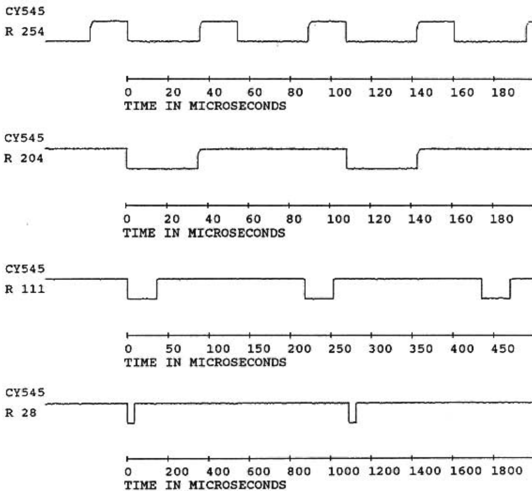
Figure 16.11 PULSE waveforms for various step rates.
